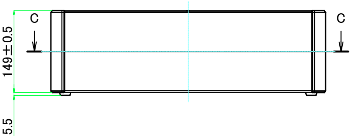
A view
