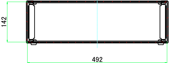
B-B (1:7)
