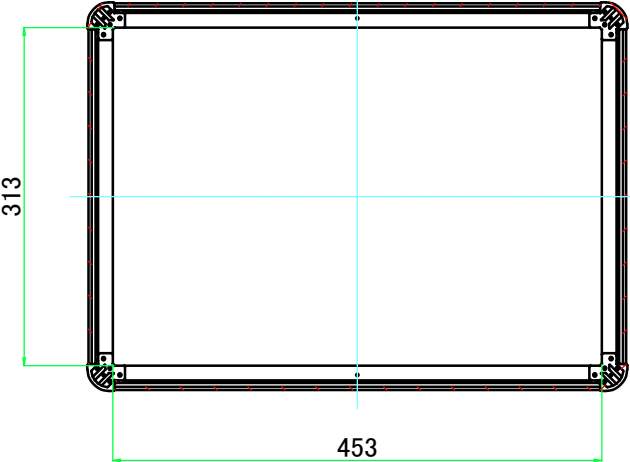
C-C (1:7)
